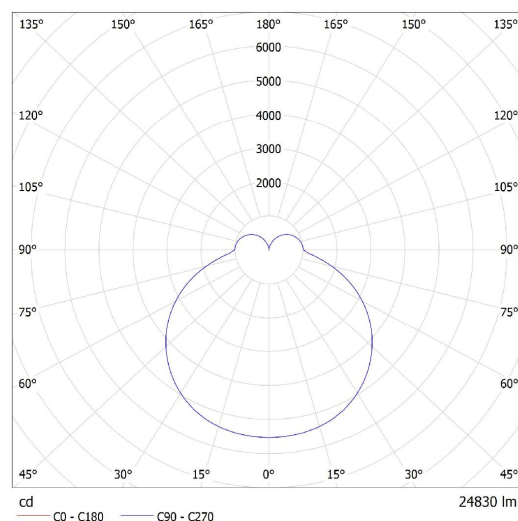
Lucis IB.L11.1250M.1 IZAR B MAX LED / LDC (Polar)
